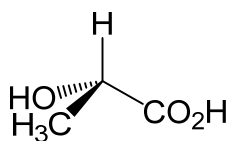
(+)-Lactic acid
